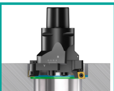
Boring Head
