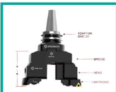
Rough Boring Heads
