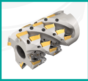
Modular Cutter
